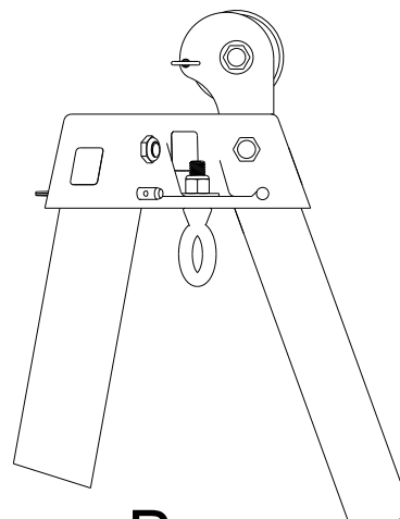
DETAIL B SCALE 3:20
